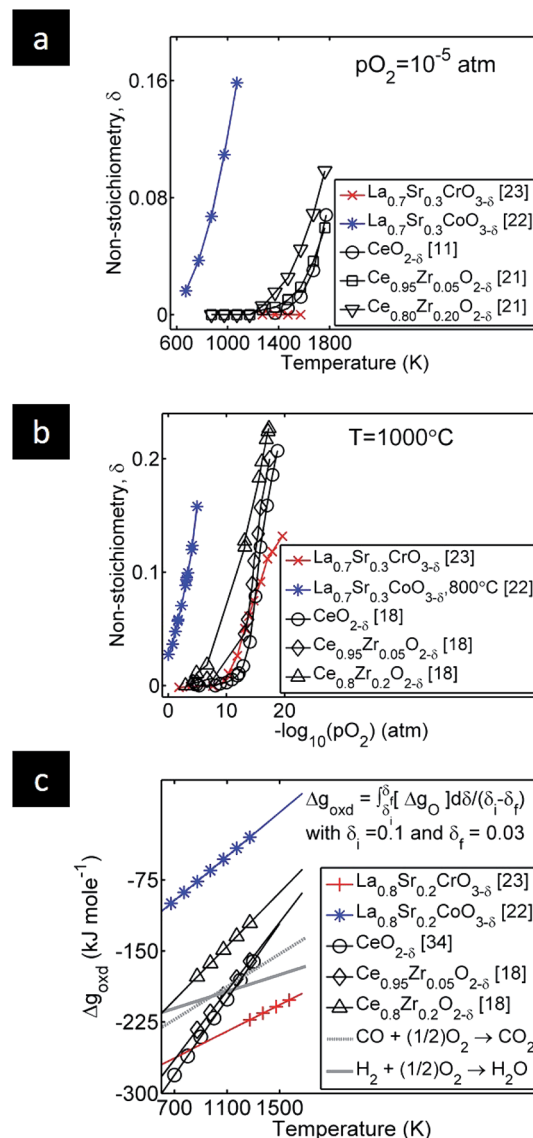
Fig. 2 Existing literature data on (\text{La,Sr})\text{BO}_{3-\delta} along with doped and pristine ceria to compare the impact of two different B-site cationic dopants: Cr and Co. (a) Non-stoichiometry vs. temperature for B-site doped \text{La}_{0.7}\text{Sr}_{0.3}\text{BO}_{3-\delta} compared to zirconia-doped ceria and pristine ceria at a constant oxygen partial pressure of p\text{O}_2 = 10^{-5} atm. Solid lines are used to guide the eye. (b) Equilibrium non-stoichiometry vs. p\text{O}_2 for B-site doped \text{La}_{0.7}\text{Sr}_{0.3}\text{BO}_{3-\delta} , zirconia-doped ceria and pristine ceria compared at a temperature of 1000 °C. The solid lines are used as guidance to the eye. (c) Gibbs free energy of oxidation, \Delta G_{\text{oxd}} , of doped perovskites compared to ceria and to the water and gas shift reaction, of relevance for the solar-to-fuel conversion, at different temperatures. The calculation of \Delta G_{\text{oxd}} is done by the integration of the oxygen molar free energy, \Delta G_{\text{O}} , for the respective materials over a realistic non-stoichiometry range: for the initial non-stoichiometry of \delta_i = 0.1 to a final non-stoichiometry of \delta_f = 0.03 . Point-markers represent the temperature range of the respective experiments and solid lines represent linear inter- and extrapolation. Information on water and \text{CO}_2 splitting is derived from NIST-JANAF thermochemical tables.
