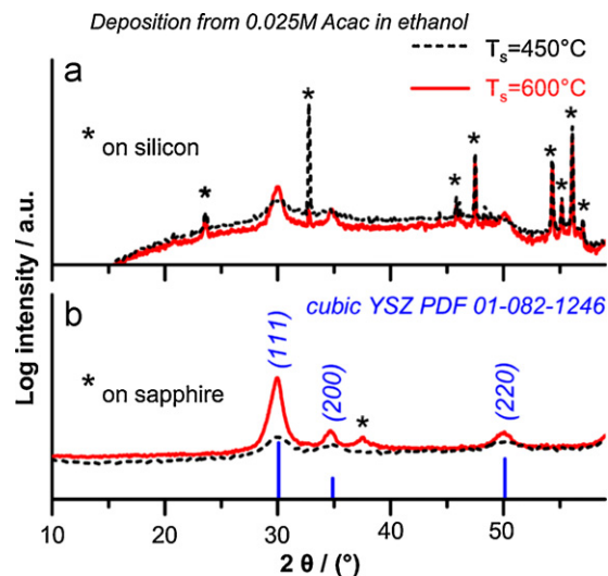
Fig. 6. Influence of substrate nature and temperature on XRD patterns of YSZ thin films. Deposition from 0.025 M \text{Zr}(\text{acac})_4 + \text{Y}(\text{acac})_3 in ethanol on (a) silicon and (b) sapphire substrates. (h k l) indices of cubic YSZ; *XRD signals of silicon and sapphire substrate, respectively.
